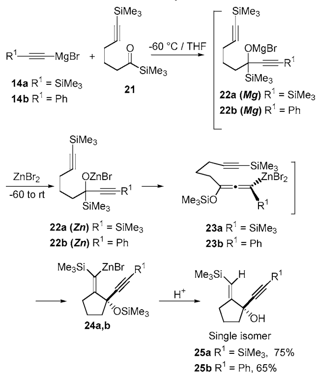
Scheme 5. Tandem Zn-Promoted Brook Followed by the Zn–Yne–Allene Carbocyclization Reaction
